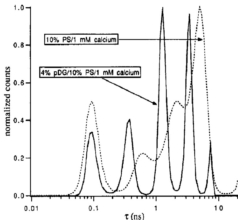
Fig. 3. Normalized inverse Laplace transforms of the fluorescence decays of PKC in a buffer containing 100 mM thesit micelles loaded with 10 mol% PS in the presence and absence of 4 mol% pDG. 100 equally spaced \tau values on a logarithmic scale between 0.01 ns and 20 ns were used in the reconstruction of the lifetime spectra by the MEM method.
