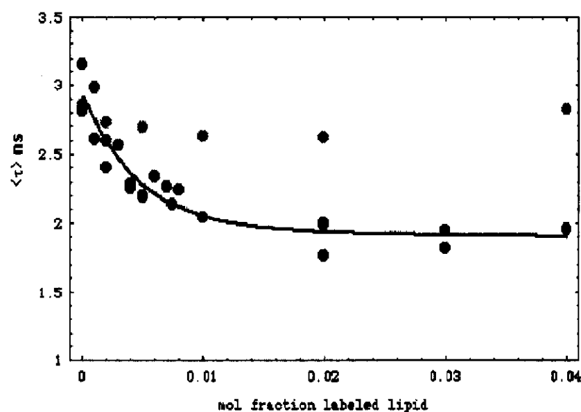
Fig. 4. Dependence of average lifetime \tau of PKC on mole fraction pDG (black circles) or pPC (gray circles) in 100 mM Thesit micelles containing 10 mol% PS. The solid curve is the best fit of eq. (9) to the pDG data by assuming a micellar size of 330 units.
